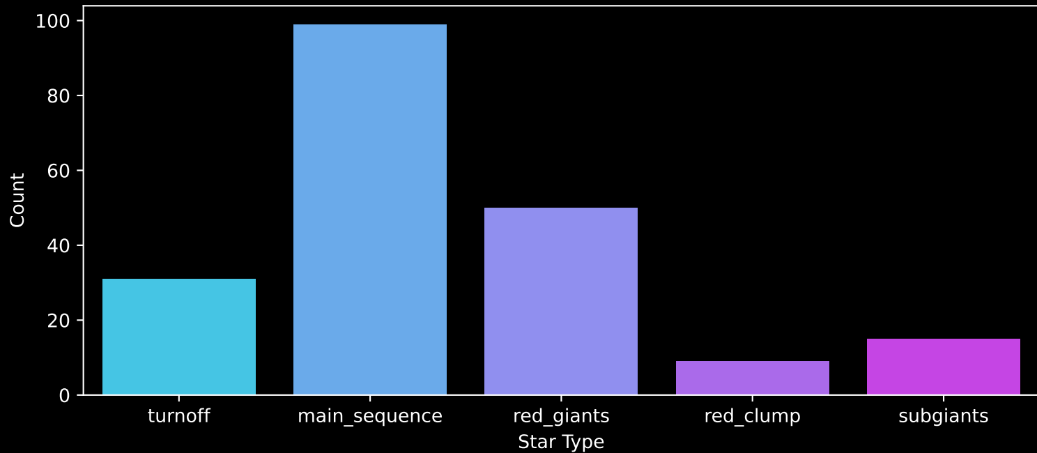
APOGEE DR17 Field: [230+32_MGA] Count plot of Star Type
