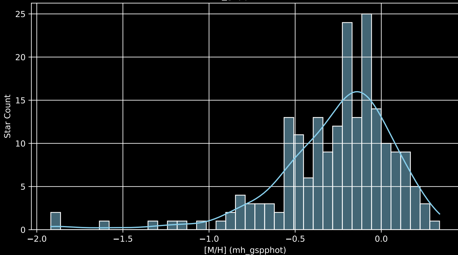
APOGEE DR17 Field: [230+32_MGA [M/H] (mh_gspphot) (n= 202)
