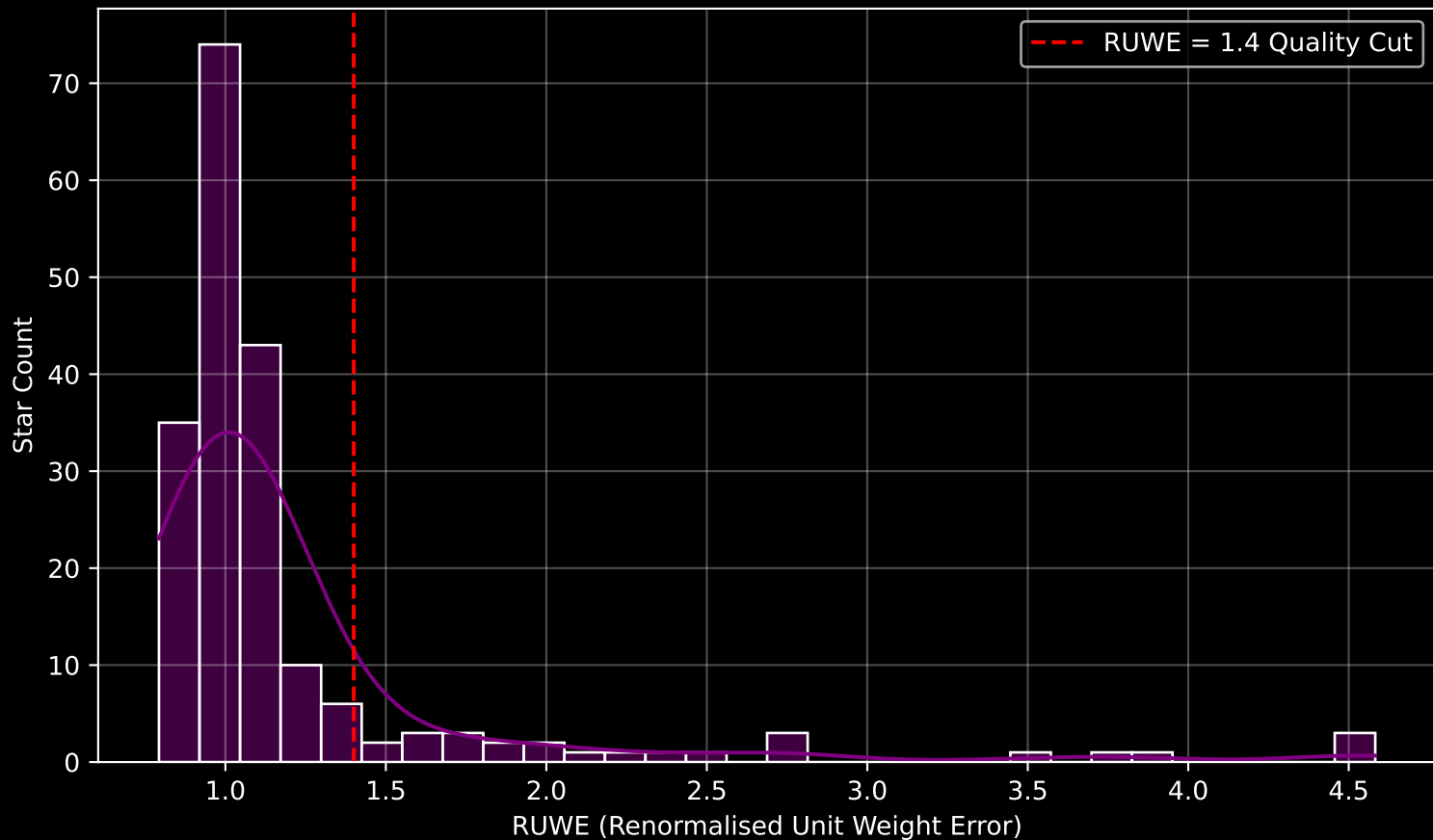
GAPOGEE DR17 Field [230+32_MGA] RUWE Distribution (n= 193)
