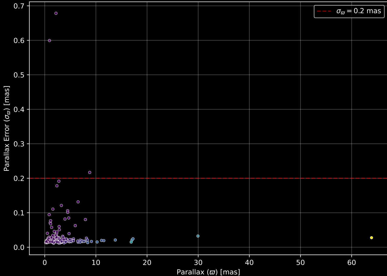
APOGEE DR17 Field: [230+32_MGA] Parallax Quality (n= 204)
