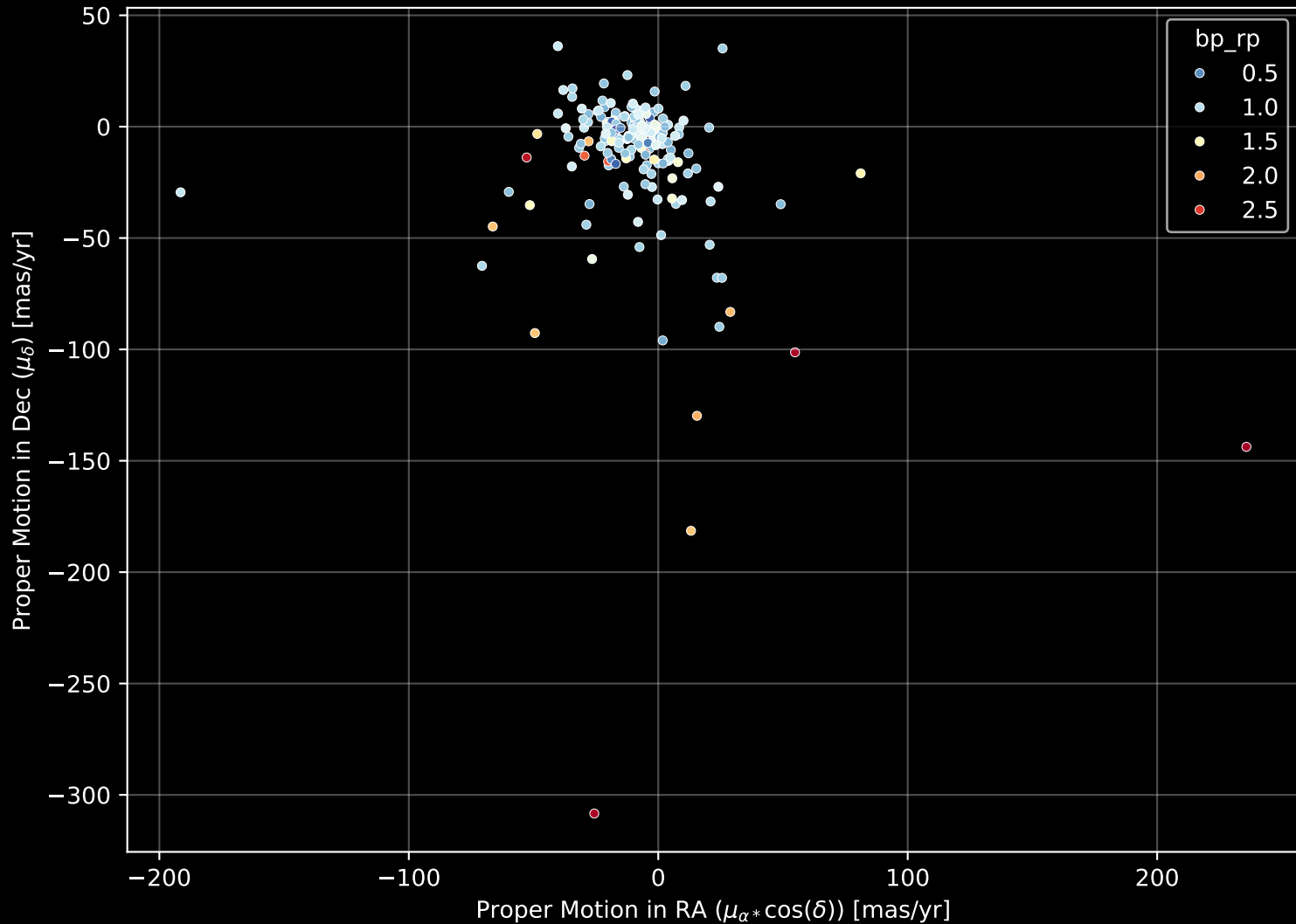
APOGEE DR17 Field: [230+32_MGA] Proper Motion Diagram (n= 204)
