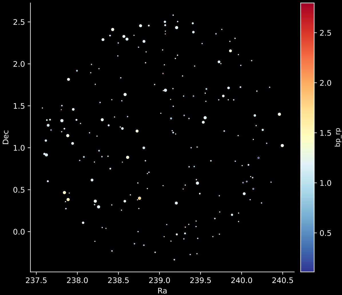
APOGEE DR17 Field: [230+32_MGA] Stars: 204
